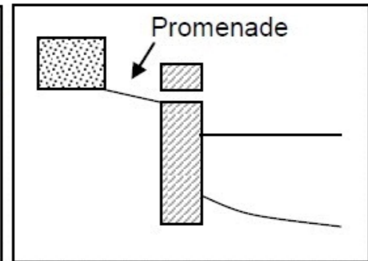
Wave return wall
