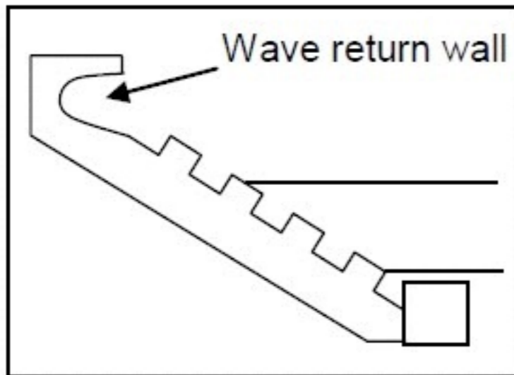
Irregular Face
